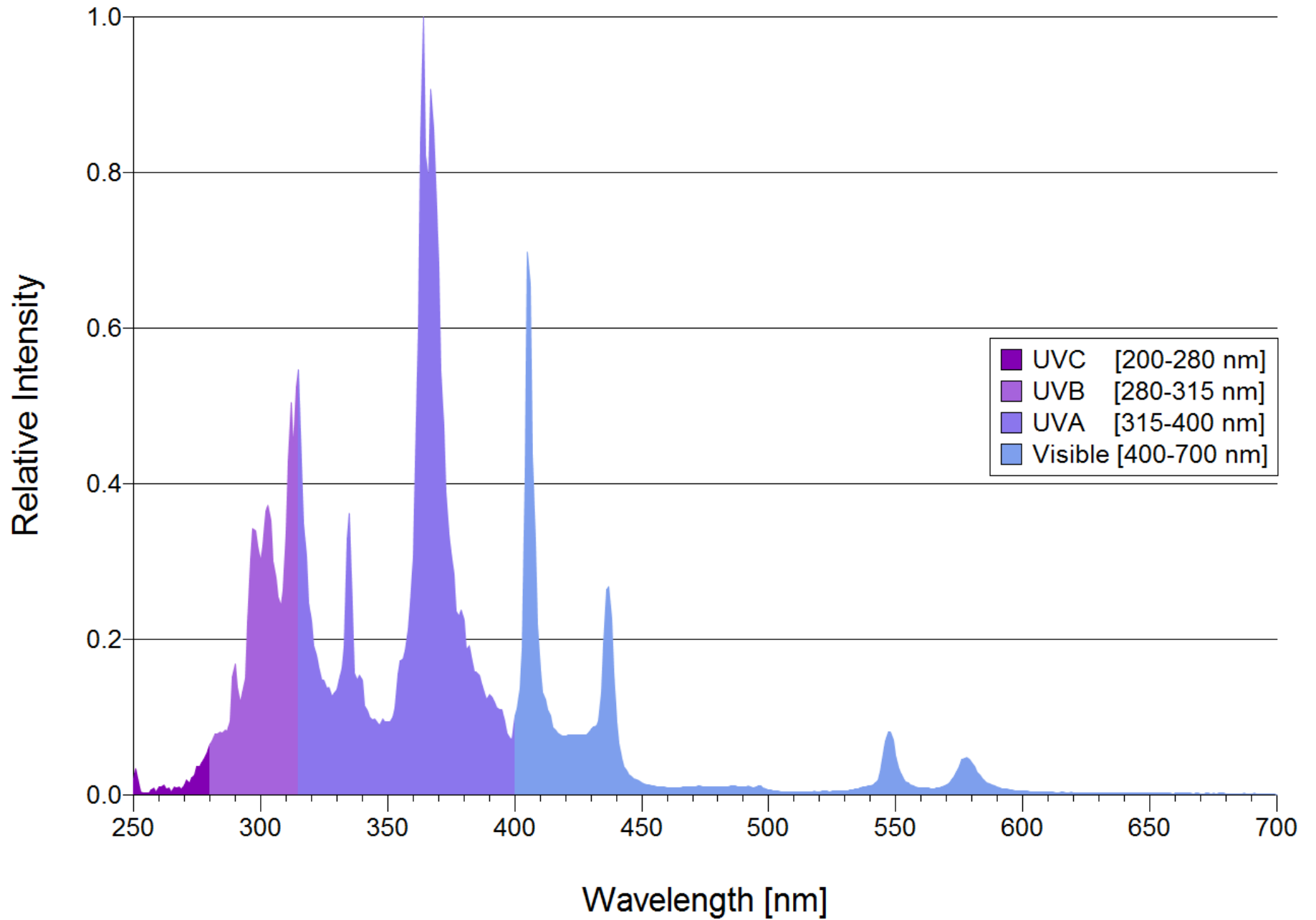
Uvitron 100W UV Enhanced Spot Lamp Spectral Distribution UV0551
