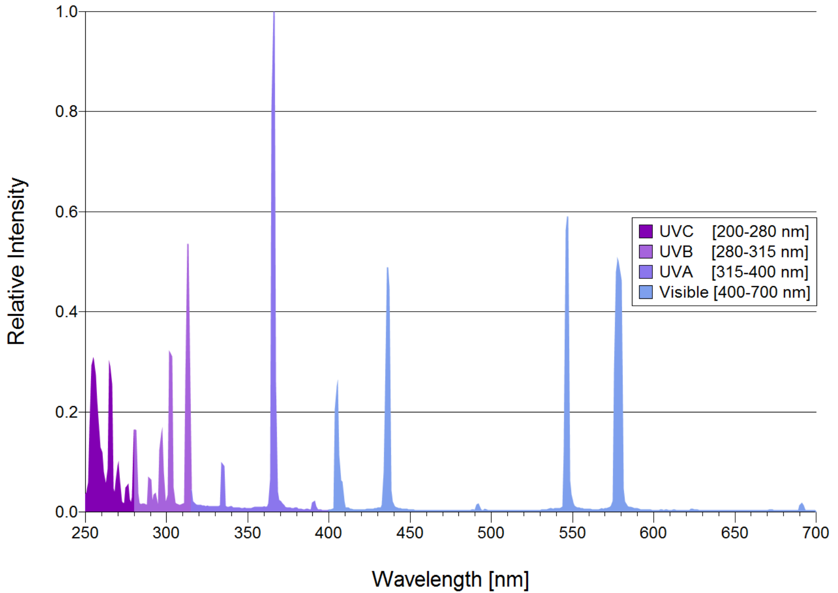
Uvitron 25" 400W/inch UVB Enhanced Lamp Spectral Distribution UV1831
