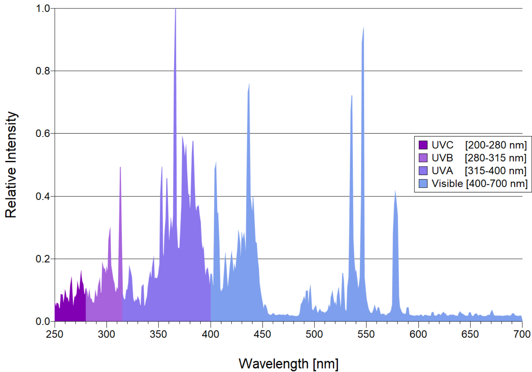
Uvitron 200W UVA Enhanced Lamp Spectral Distribution UV1228
