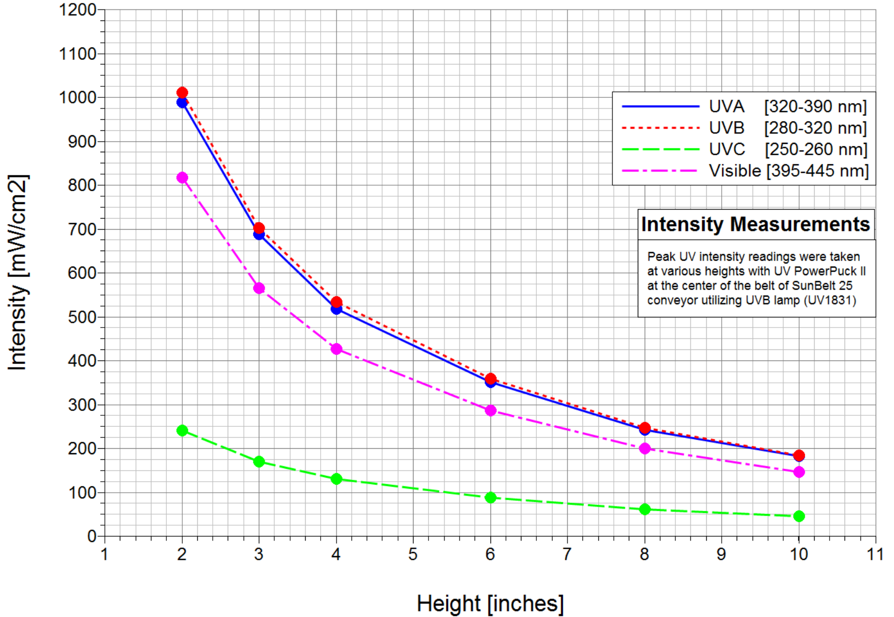
SunBelt 25, UVB Lamp Intensity vs. Height
