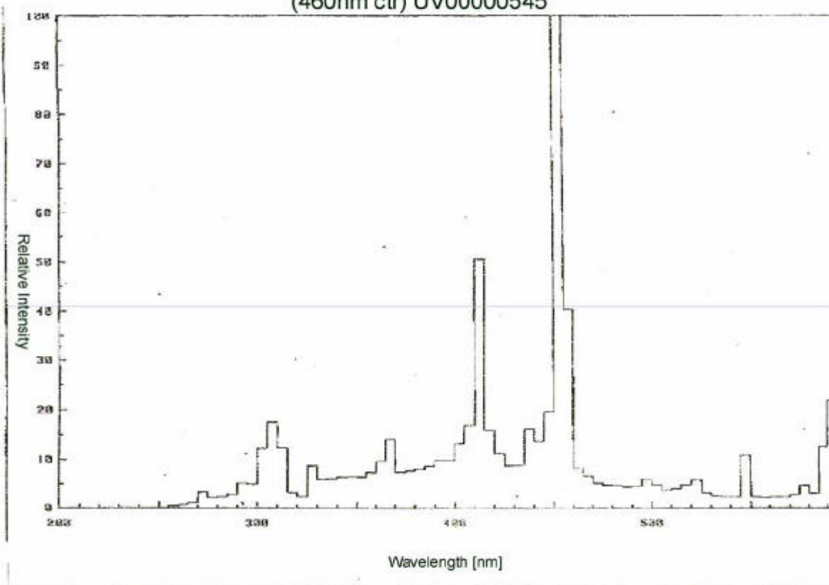
Uvitron 400W Visible Enhanced Lamp Spectral Distribution (460nm ctr) UV00000545
