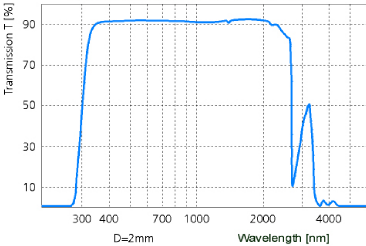
Uvitron Short Wave Filter Transmission Curve
